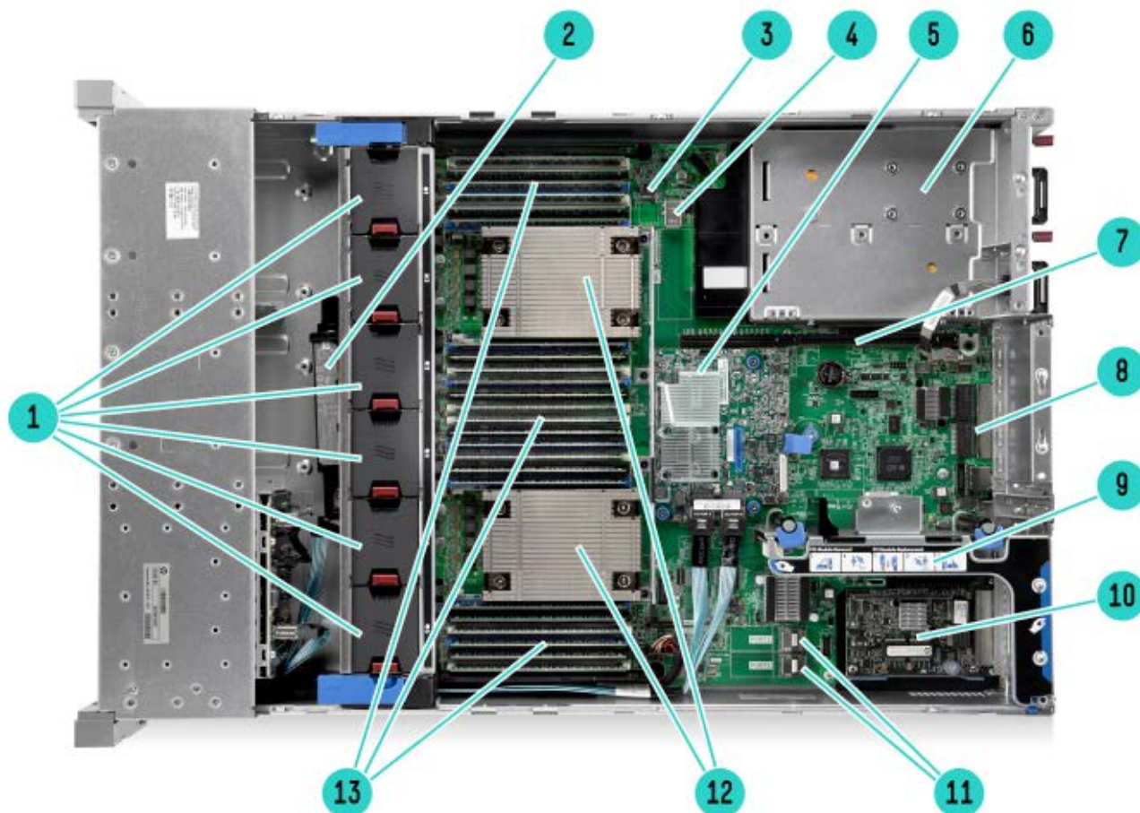
Internal View
